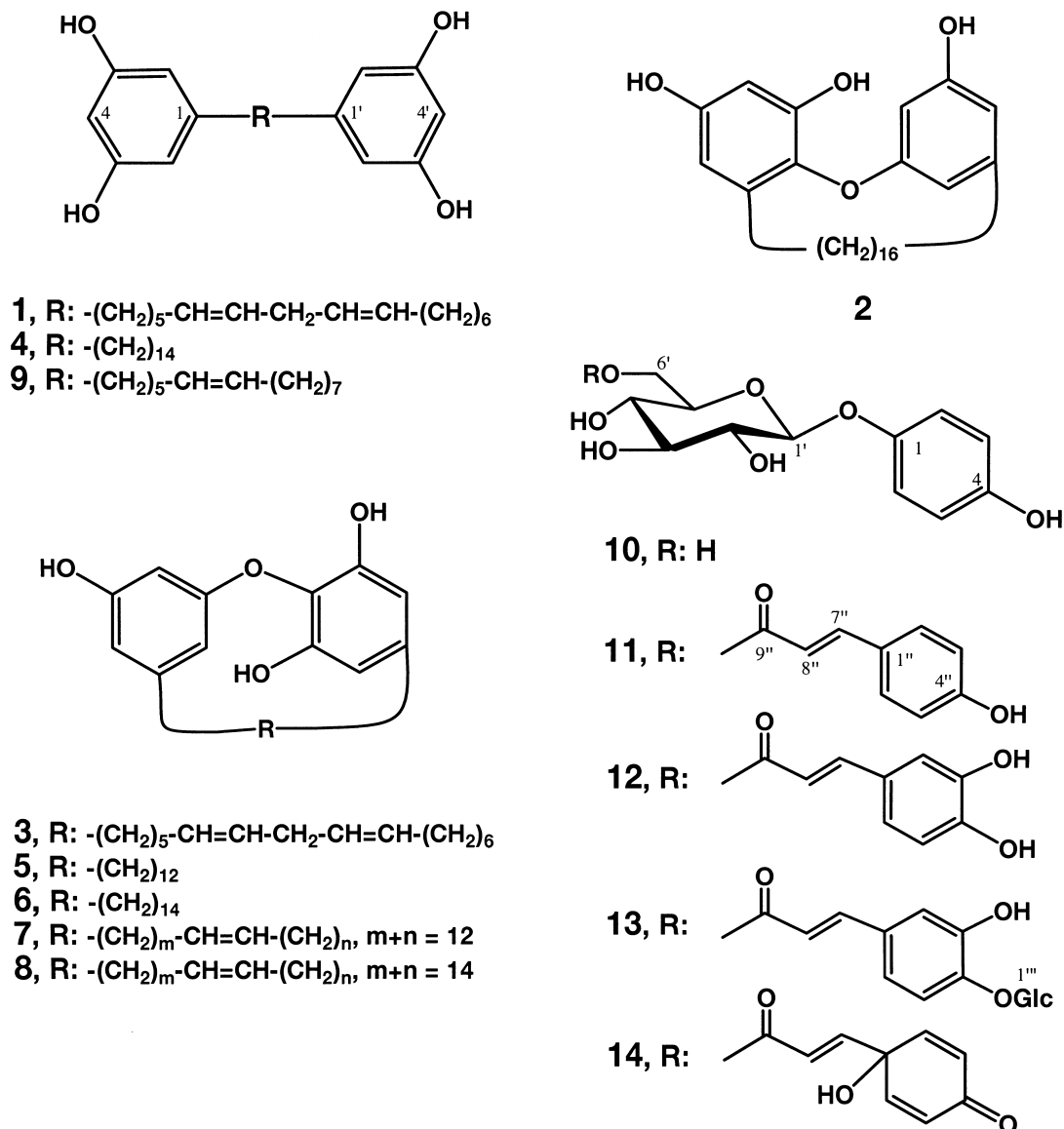
Fig. 1. Phenolic compounds isolated from G. robusta .
